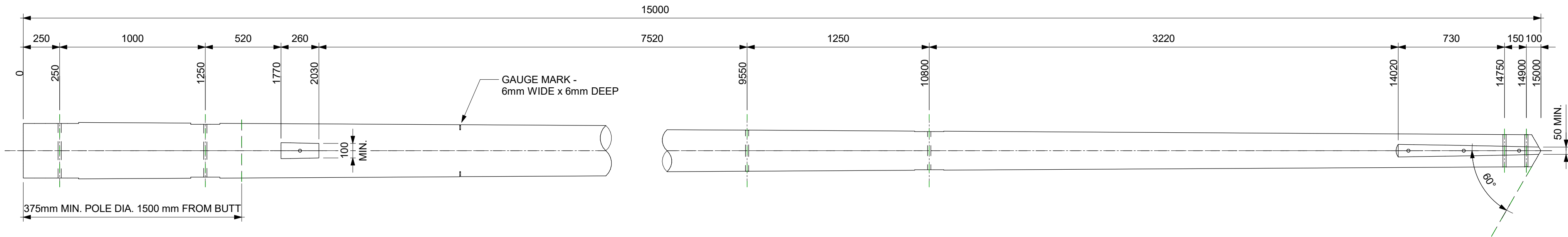
Elevation Side
